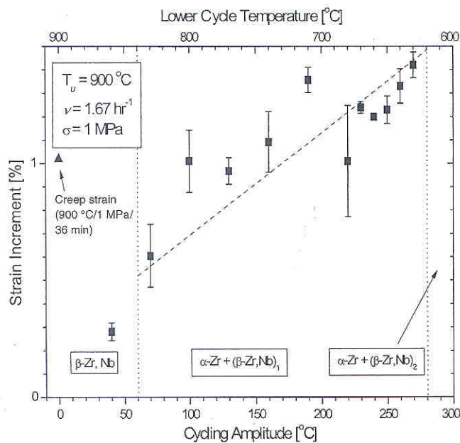
Fig. 4 Strain increment per cycle as a function of cycling amplitude ( T_u - T_l ) at constant upper temperature T_u = 900\text{ }^\circ\text{C} ( \nu = 1.67\text{ h}^{-1} , \sigma = 1\text{ MPa} ). Also shown is the calculated creep strain accumulated during 36 min (a full cycle) at T_u .
