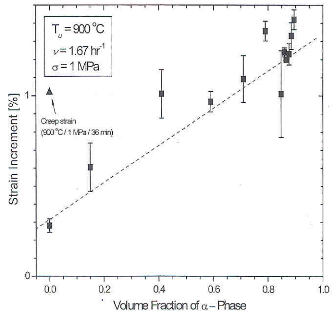
Fig. 7 Strain increment per cycle (experimental data from Fig. 4) as a function of estimated volume fraction of transformed \alpha -Zr
