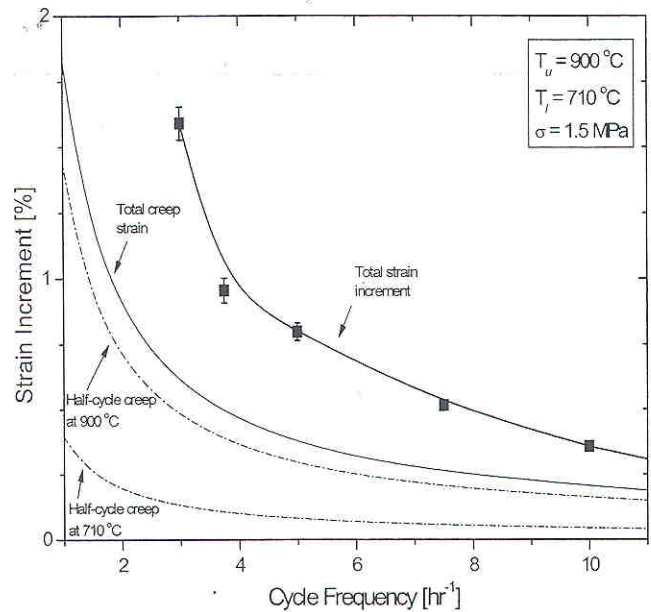
Fig. 5 Strain increment per cycle as a function of cycling frequency ( T_l = 710\text{ }^\circ\text{C} , T_u = 900\text{ }^\circ\text{C} , \sigma = 1.5\text{ MPa} ). Also shown are calculated creep strains accumulated during a half cycle at T_l and T_u and their sum.
