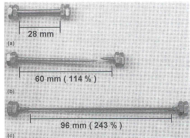
Fig. 6 Zr-705 specimens. (a) Before deformation. (b) After isothermal creep deformation at 900\text{ }^\circ\text{C} ( \sigma = 0.5 to 8.2\text{ MPa} ), showing fracture. (c) After superplastic deformation by thermal cycling between 710 and 900\text{ }^\circ\text{C} ( \sigma = 1.5 to 2\text{ MPa} , \nu = 3\text{ h}^{-1} ), showing no fracture
