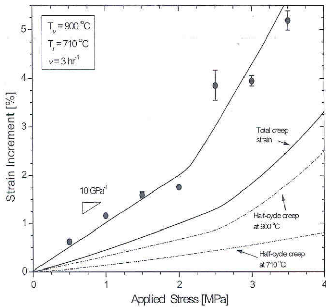
Fig. 3 Strain increment per cycle as a function of applied stress ( T_l = 710\text{ }^\circ\text{C} , T_u = 900\text{ }^\circ\text{C} , \nu = 3\text{ h}^{-1} ). Also shown are calculated creep strains accumulated during 10 min (a half cycle) at T_l and T_u and their sum.
