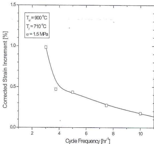
Fig. 8 Corrected strain increment per cycle (experimental data from Fig. 5 to which the creep strain was subtracted) as a function of cycling frequency ( T_l = 710 °C, T_u = 900 °C, \sigma = 1.5 MPa)
