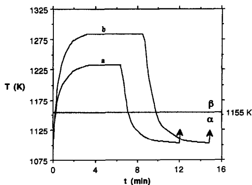
Fig. 1. Experimental thermal cycles: (a) low temperature cycle and (b) high temperature cycle.
