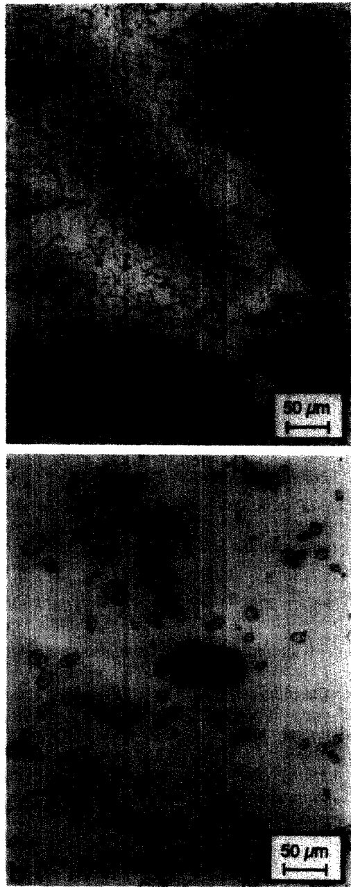
Fig. 2. Micrographs of undeformed (a) CP-Ti (Kroll's reagent) and (b) Ti-TiC (unetched).
