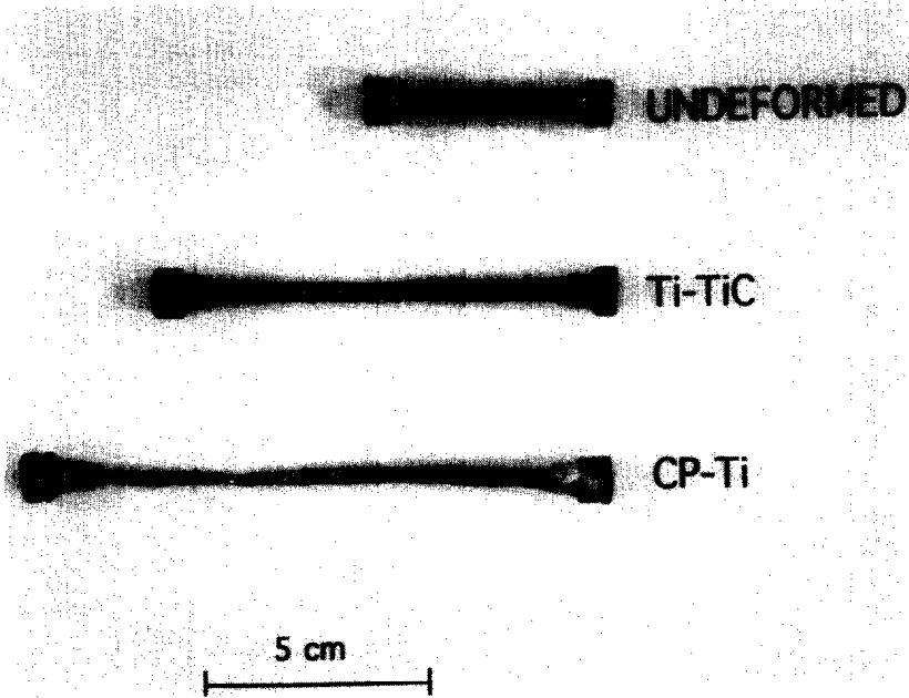
Fig. 6. Thermally-cycled samples deformed to fracture. CP-Ti: 200% strain for a stress of 1.4 \pm 0.2 MPa. Ti-TiC: 135% strain for a stress of 1.25 \pm 0.05 MPa.
