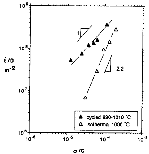
Fig. 10. Normalized strain rates as a function of stress for Ti-TiC deformed under cycling and isothermal conditions.
