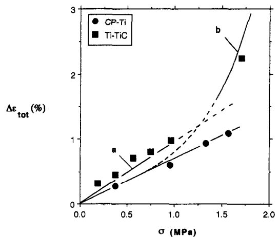
Fig. 11. Total strain per cycle \Delta\epsilon_{\text{tot}} as a function of applied stress \sigma , measured for CP–Ti and Ti–TiC cycled between 830 and 1010°C. Predicted strain for Ti–TiC (a) at low stresses from equations (12a) and (17) and (b) at high stresses from equations (12b) and (17).
